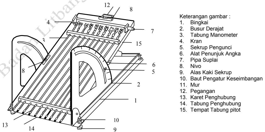
Gambar A.3 Manometer
